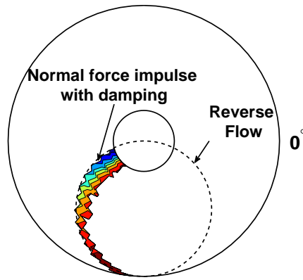
(a) \Delta C_N .
