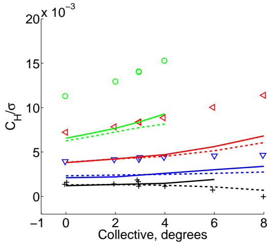
(c) H-force coefficient, C_H/\sigma .
