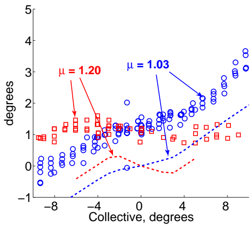
(c) \theta_{1C}, \mu > 0.825 .
