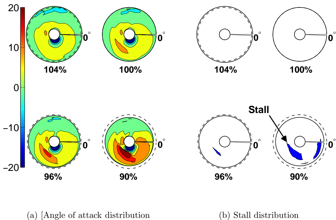
Figure 2.11: Angle of attack and stall locus at 120 knots ( W = 18,000 lb) (Disc area is scaled to represent the radius and the dashed circle indicates the baseline rotor)
