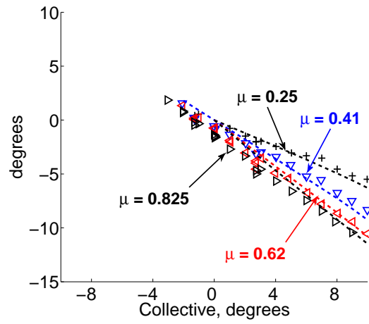
(b) \theta_{1S}, \mu \leq 0.825 .
