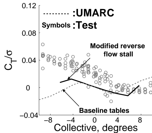
(b) Thrust reversal at \mu = 1.03 .
