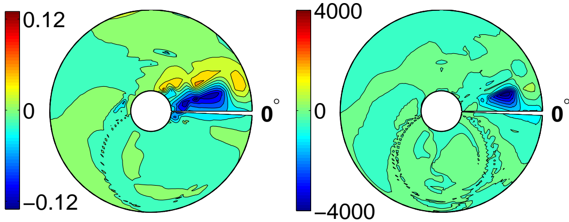
(a) Change in inflow velocity ( \Delta\Omega R ). (b) Change in shaft power, \text{ft}\cdot\text{lb}\cdot\text{s}^{-1}/\text{ft} .
