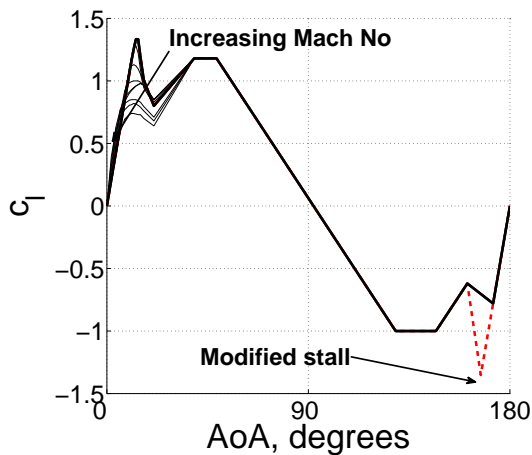
(a) Modified NACA0012 airfoil tables.
