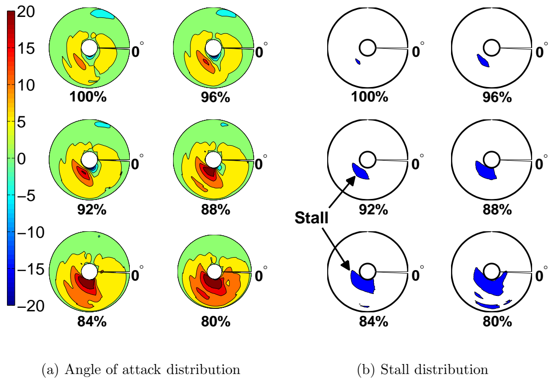
Figure 3.7: Angle of attack and stall locus for 18,000 lb thrust case at 80 knots with RPM variation.
