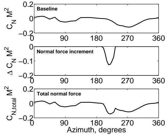
(b) Normal force at 30% radius.
