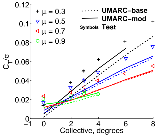
(a) Thrust coefficient, C_T/\sigma .
