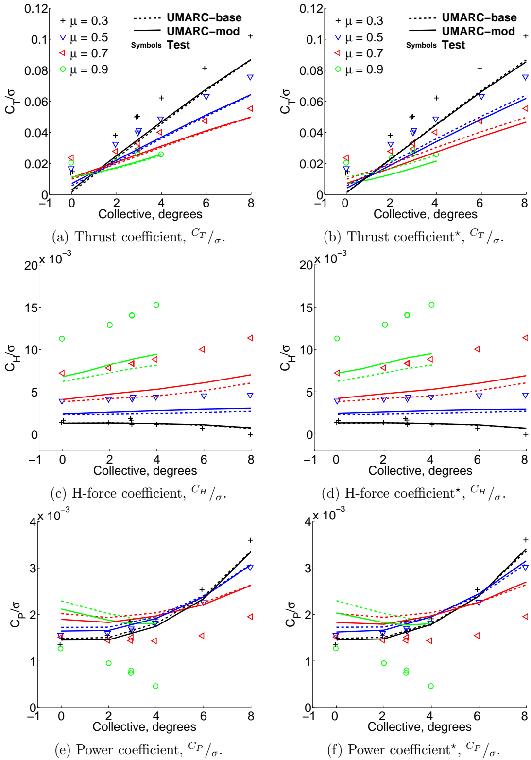
Figure 4.19: Effect of fuselage on performance predictions, M_{tip} = 0.26 , 0^\circ shaft angle (Symbols: Test, - - : Baseline analysis, — : Modified analysis, left-hand figures are upwash only (front of rotor), right-hand figures (*) are complete fuselage model).
