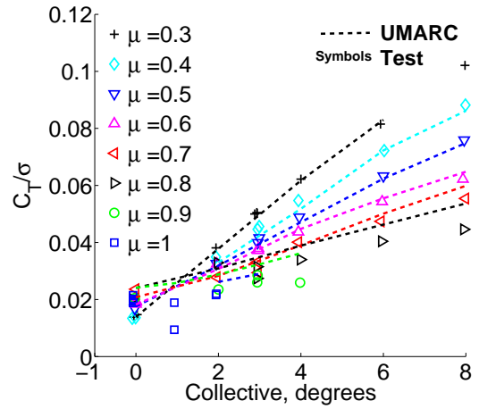
(b) Thrust coefficient + \Delta C_T/\sigma = 0.009 .
