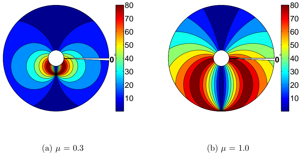
Figure 4.14: Radial flow angles (degrees) around the azimuth at high advance ratio.
