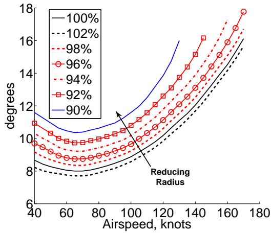
(a) Collective, \theta_0
