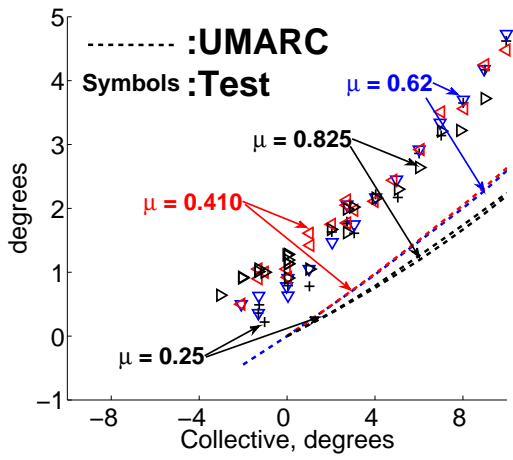
(a) \theta_{1C}, \mu \leq 0.825 .
